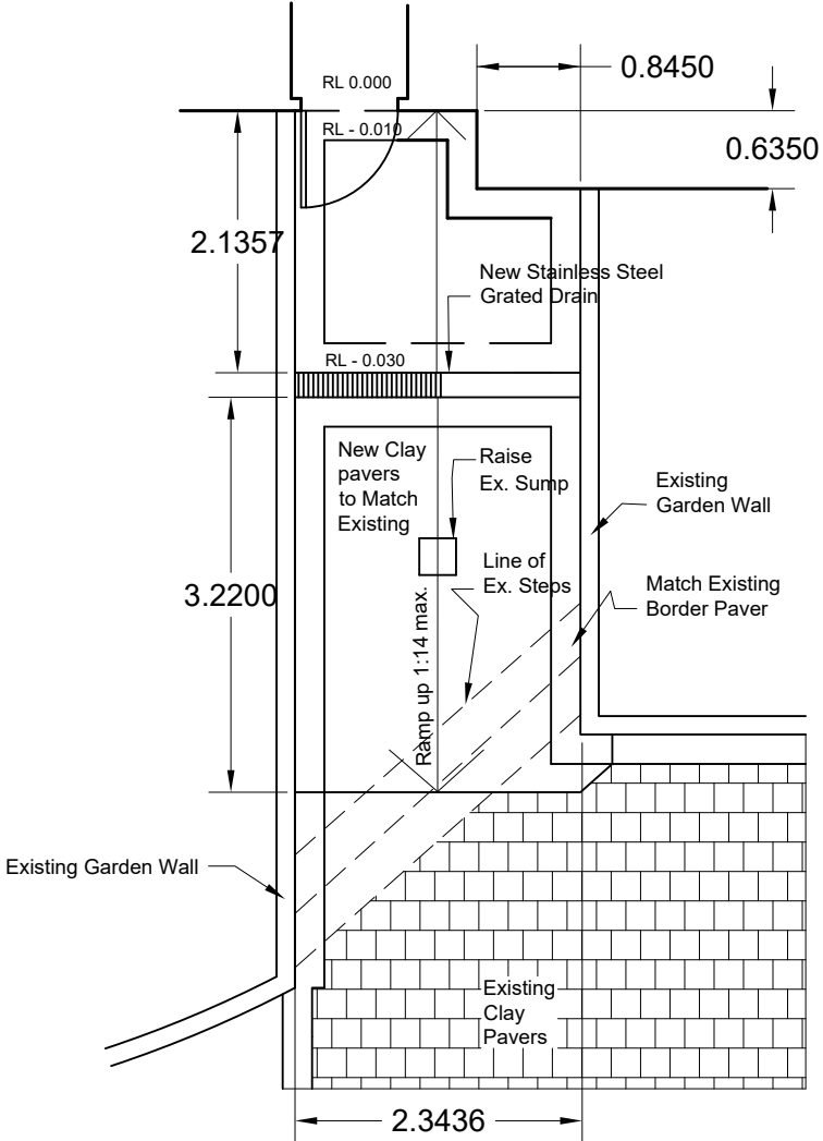
PLAN
